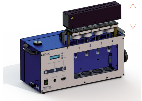
Dynamic opening cabinet of HAGUE 7000
